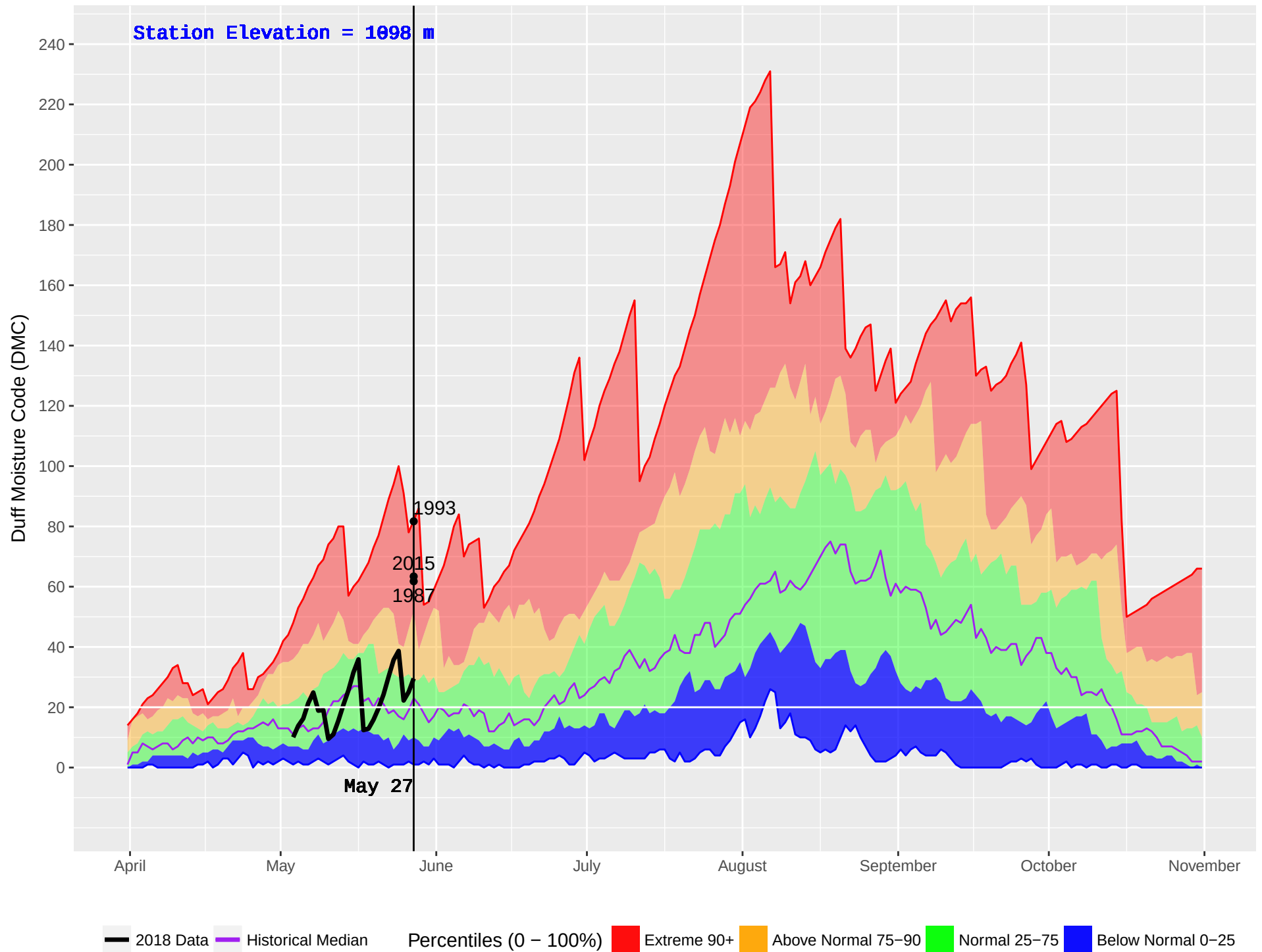
GOATFELL (401) : Historical (1986–2016) and Current (2018) Noon Duff Moisture Code (DMC)
