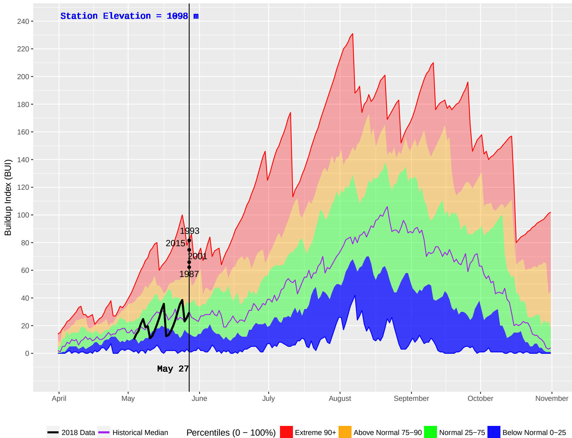
GOATFELL (401) : Historical (1986–2016) and Current (2018) Noon Buildup Index (BUI)
