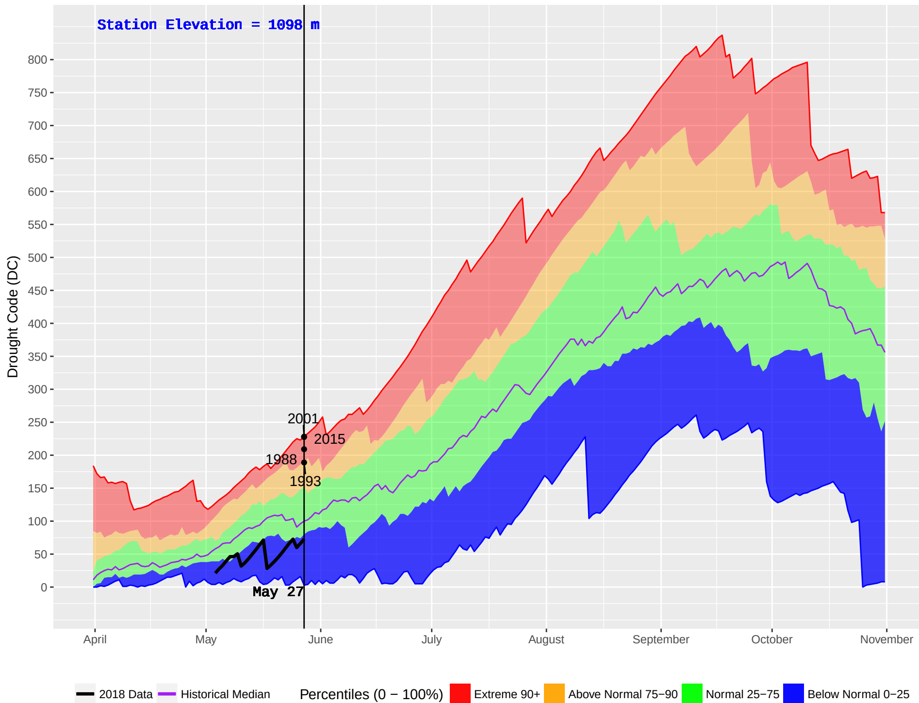
GOATFELL (401) : Historical (1986–2016) and Current (2018) Noon Drought Code (DC)
