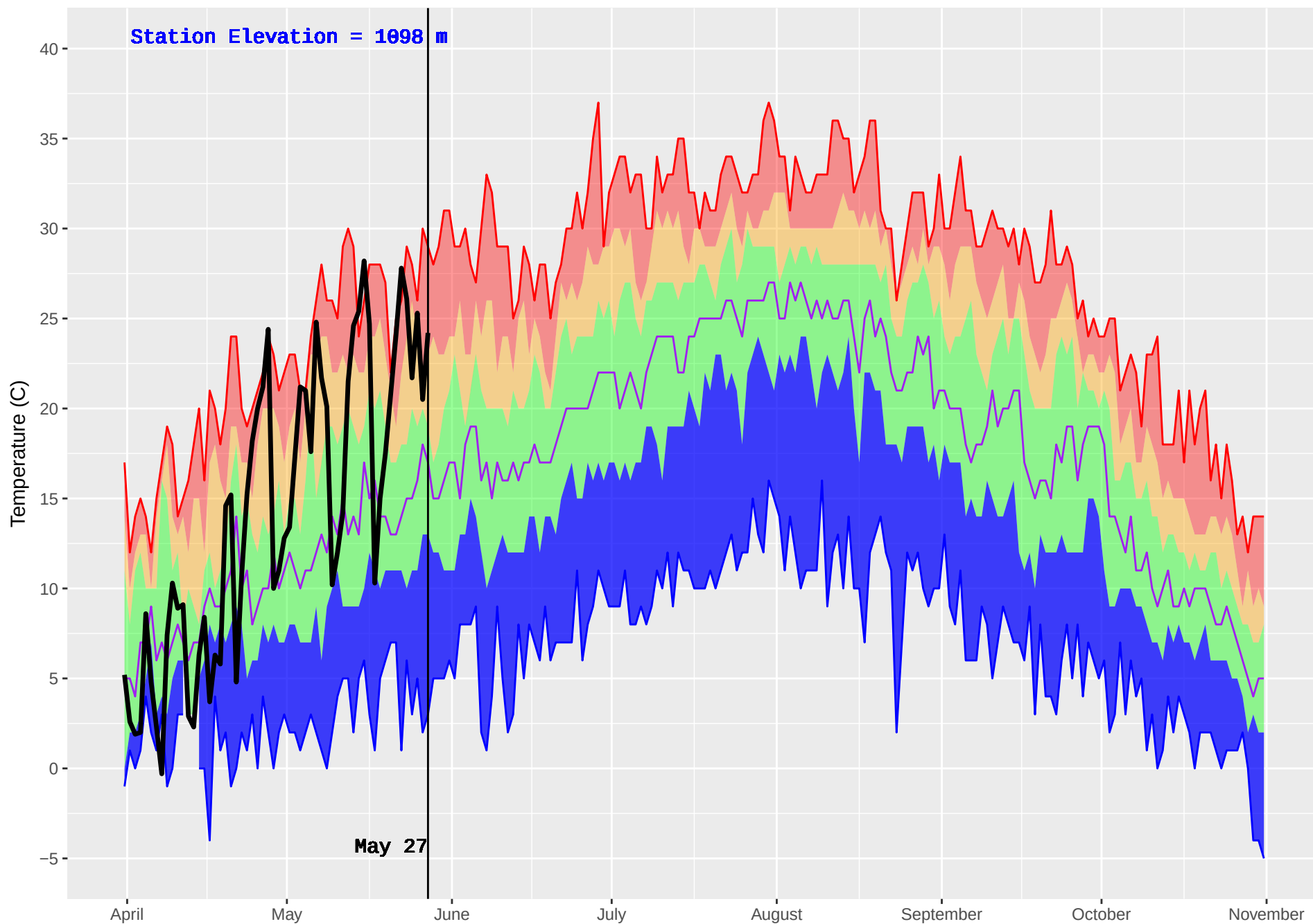
GOATFELL (401) : Historical (1986–2016) and Current (2018) Noon Temperature
