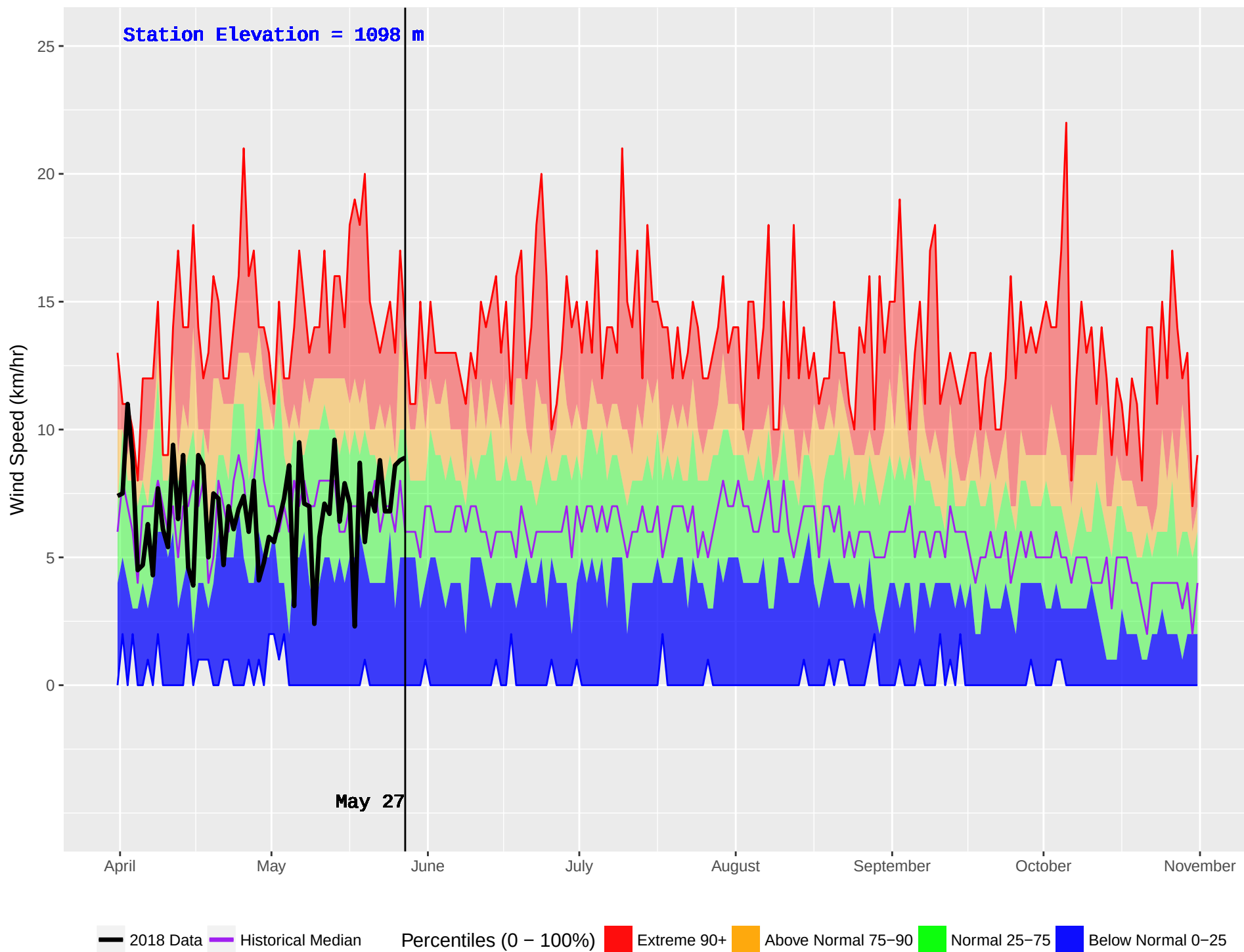
GOATFELL (401) : Historical (1986–2016) and Current (2018) Noon Wind Speed
