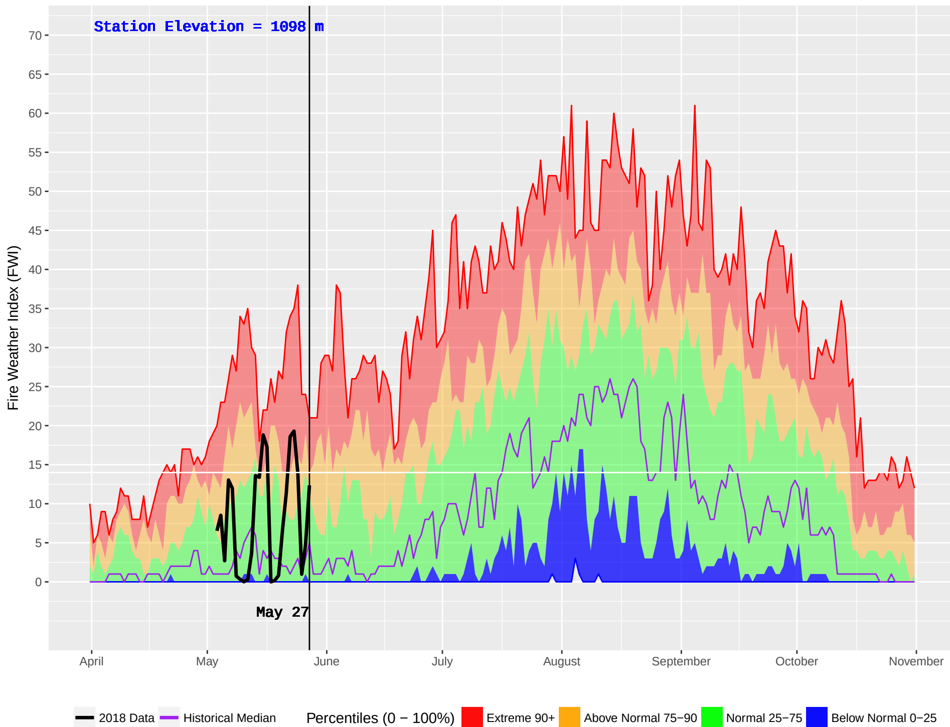
GOATFELL (401) : Historical (1986–2016) and Current (2018) Noon Fire Weather Index (FWI)
