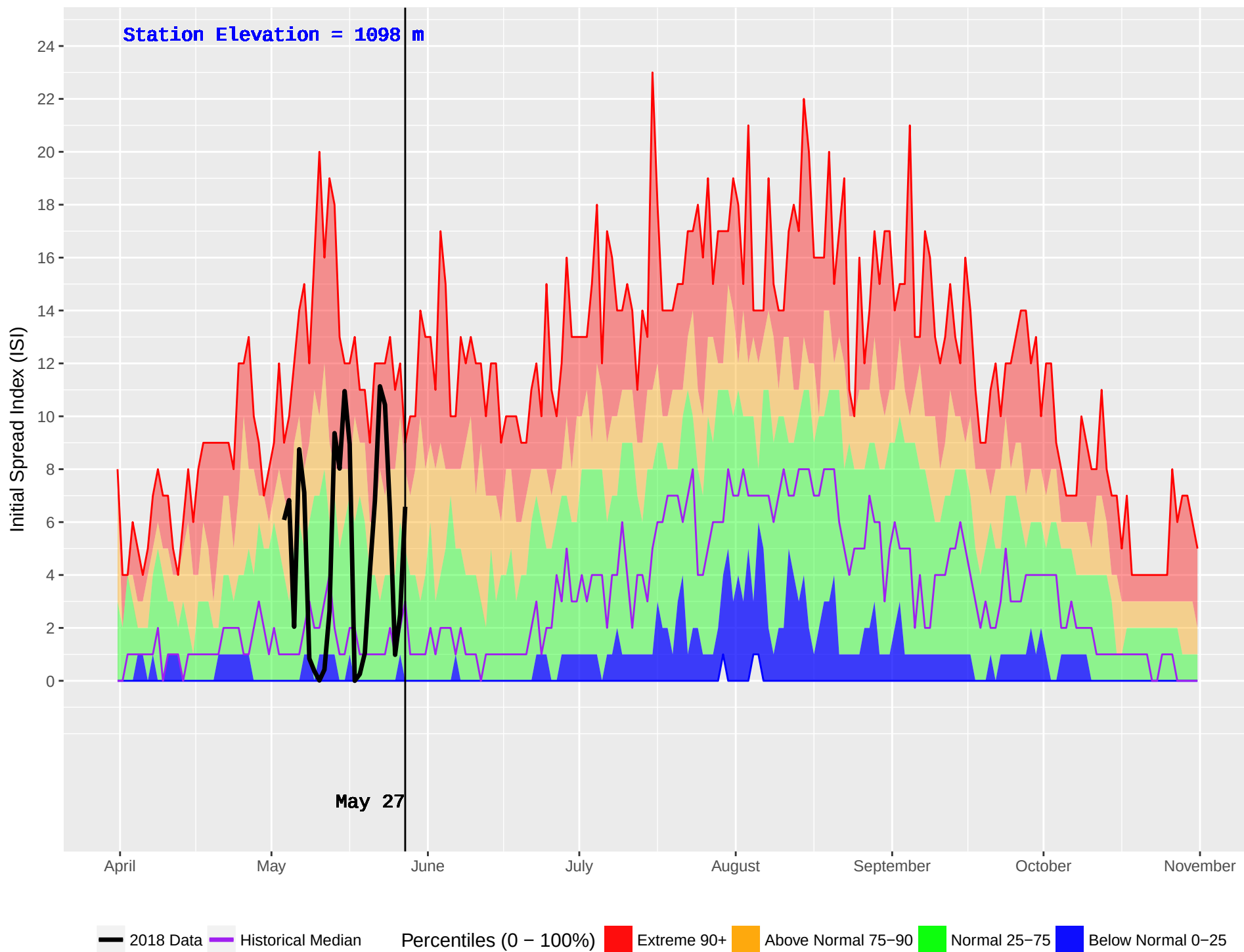
GOATFELL (401) : Historical (1986–2016) and Current (2018) Noon Initial Spread Index (ISI)
