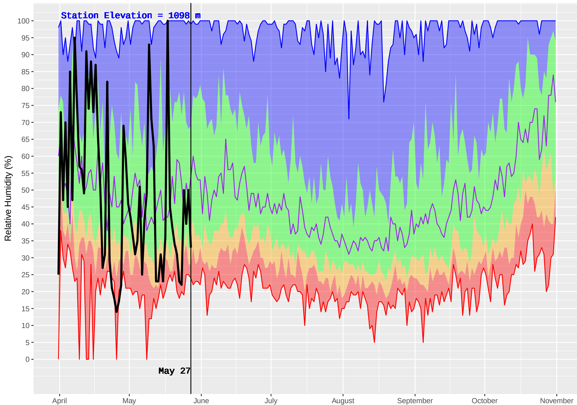
GOATFELL (401) : Historical (1986–2016) and Current (2018) Noon Relative Humidity
